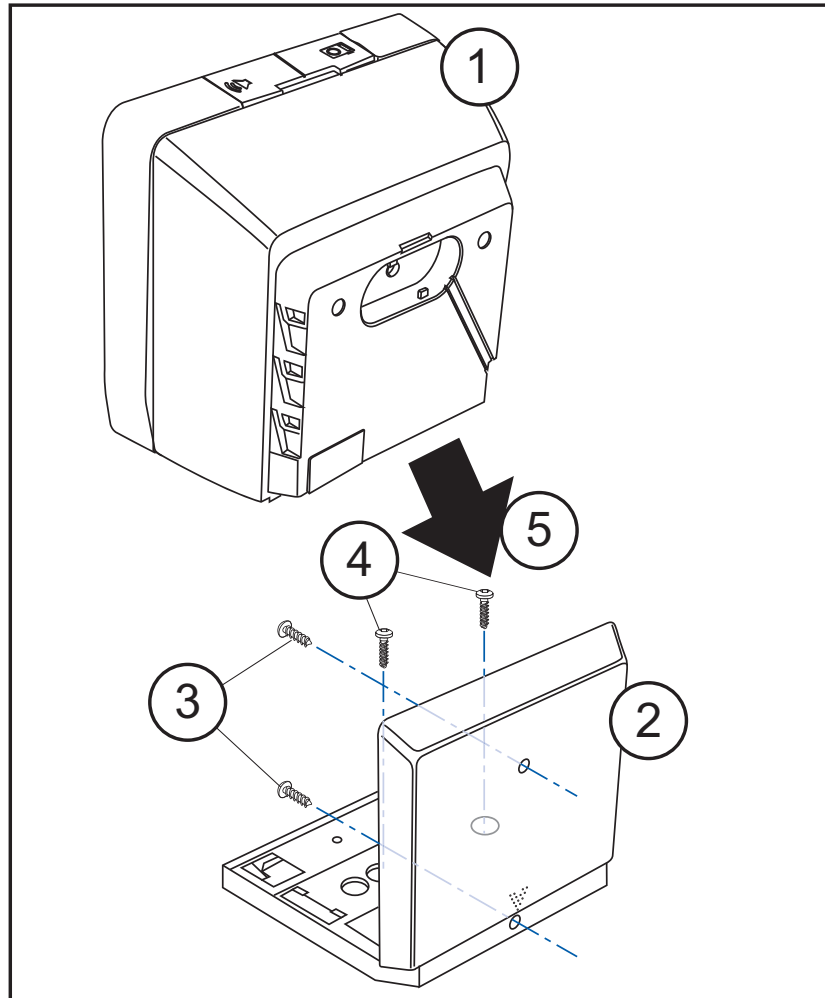
Figure 3. L-Bracket Mount
