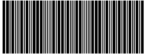
Code 2 of 5
